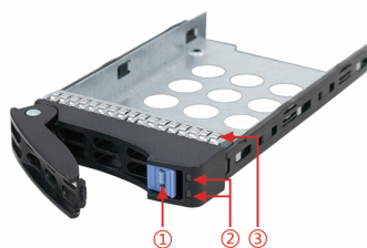
①. Lock catch ②. HDD LED ③. Anti-EMI design
