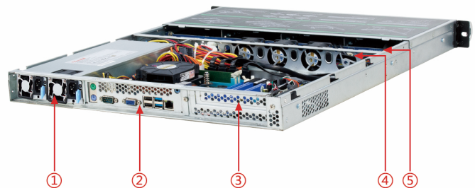
①. Redundant Power Supply
